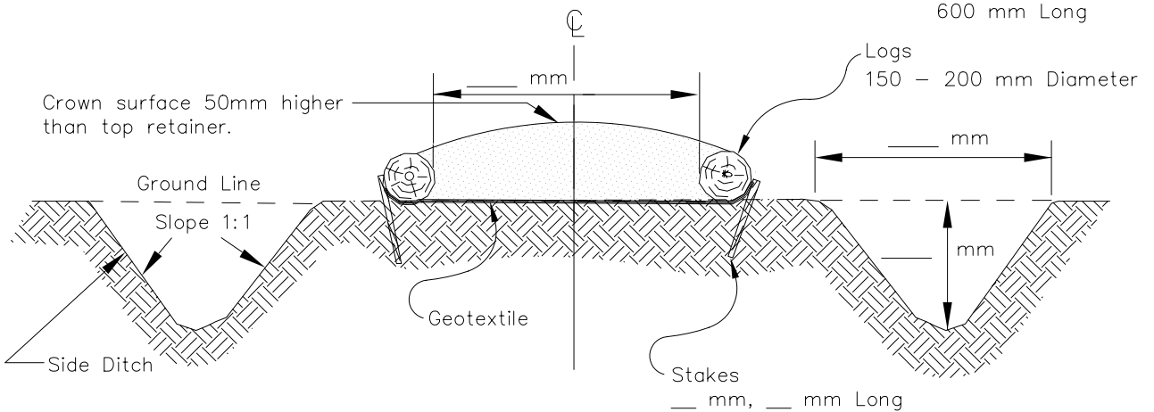
CROSS SECTION
